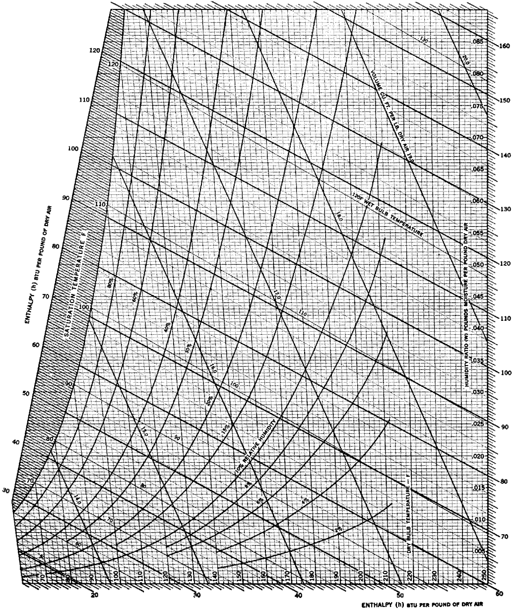
Figure 1.8 Psychrometric Chart - High Temperature
