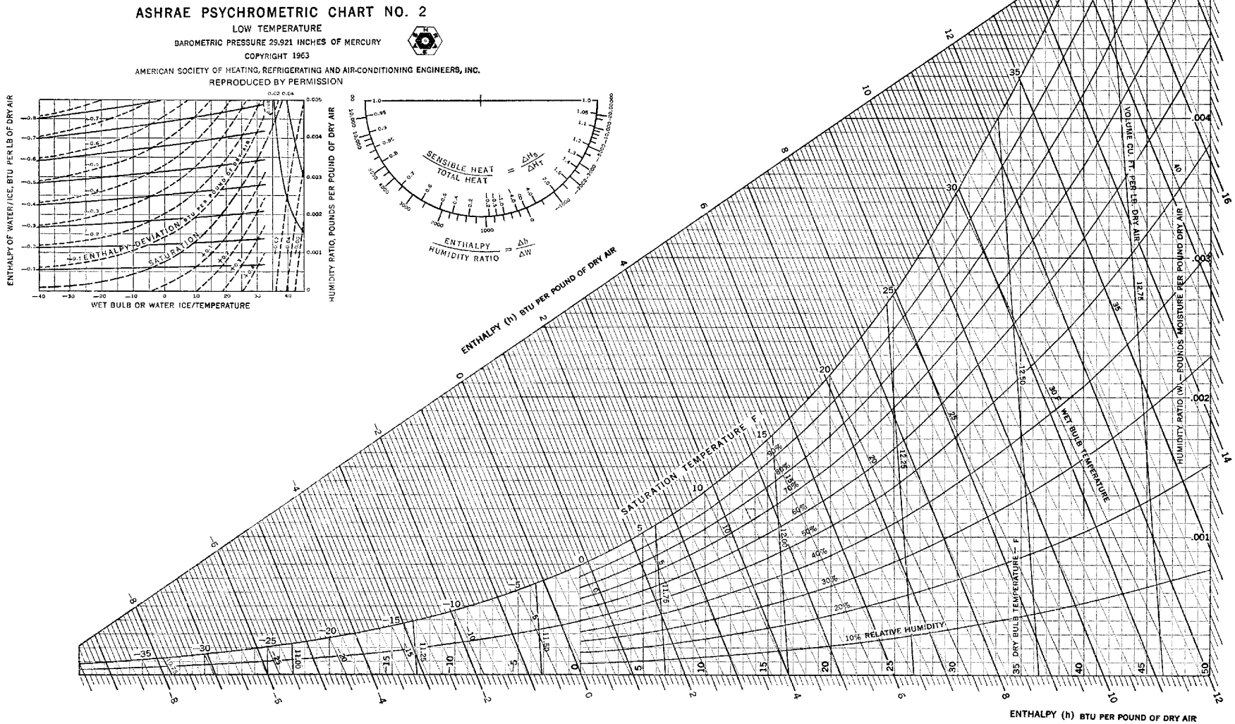
Figure 1.7 Psychrometric Chart - Low Temperature
