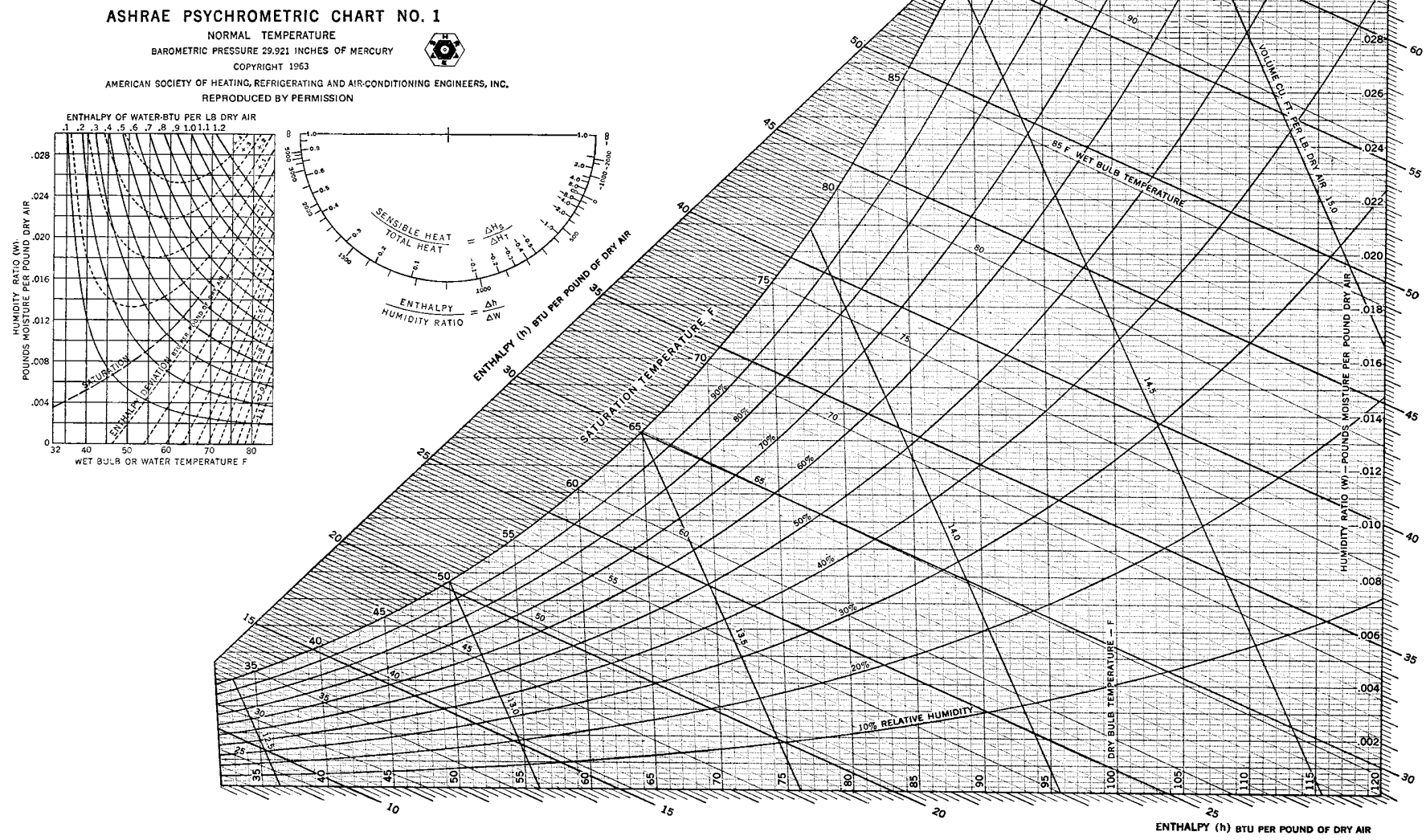
Figure 1.6 Psychrometric Chart - Standard
