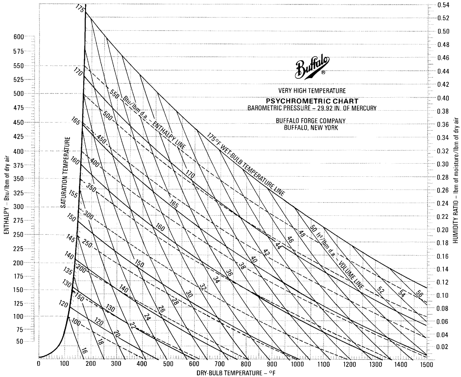
Figure 1.9 Psychrometric Chart - Very-High Temperature
