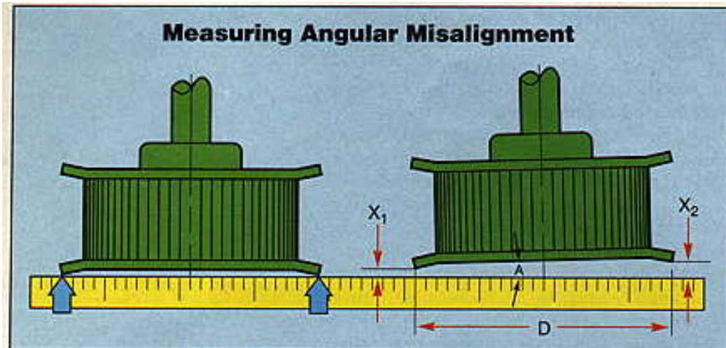
Fig. 4. Angular misalignment is corrected by moving one of the members in a drive train, usually the driver or motor.
