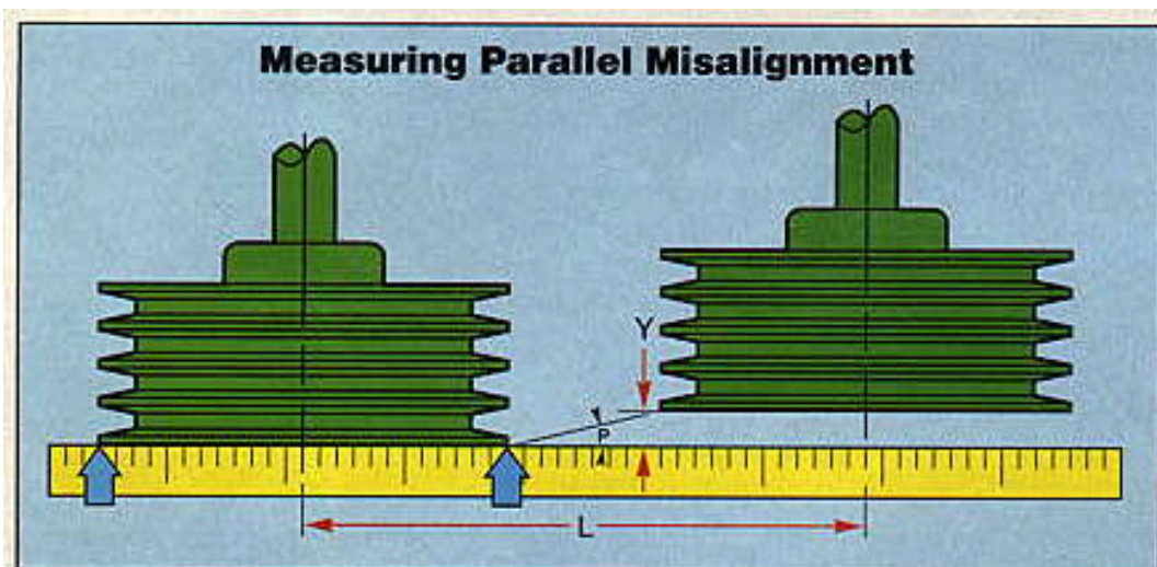
Fig. 5. Parallel misalignment is corrected by adjusting sheaves and sprockets on one or both shafts in a drive train.
