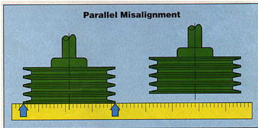
Fig. 2. Parallel misalignment causes noise, tooth and sprocket wear, poor tracking, and excessive temperatures.
